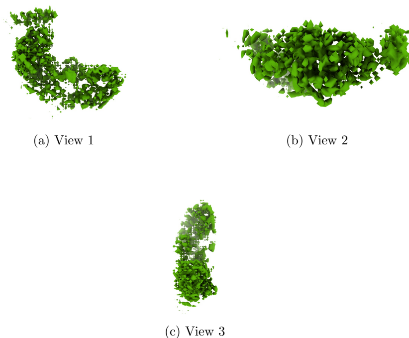
Figure 4: Isosurface at threshold=0.085400. Views generated by ChimeraX at a the following X, Y, Z angles: View 1 (0, -90, -90), View 2 (-90, 0, -90), View 3 (0, 0, 0).
