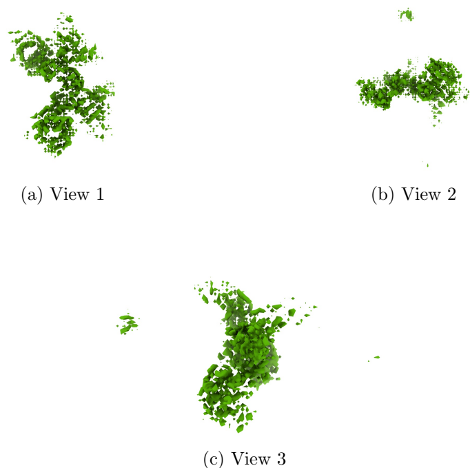
Figure 4: Isosurface at threshold=0.103000. Views generated by ChimeraX at a the following X, Y, Z angles: View 1 (0, -90, -90), View 2 (-90, 0, -90), View 3 (0, 0, 0).
