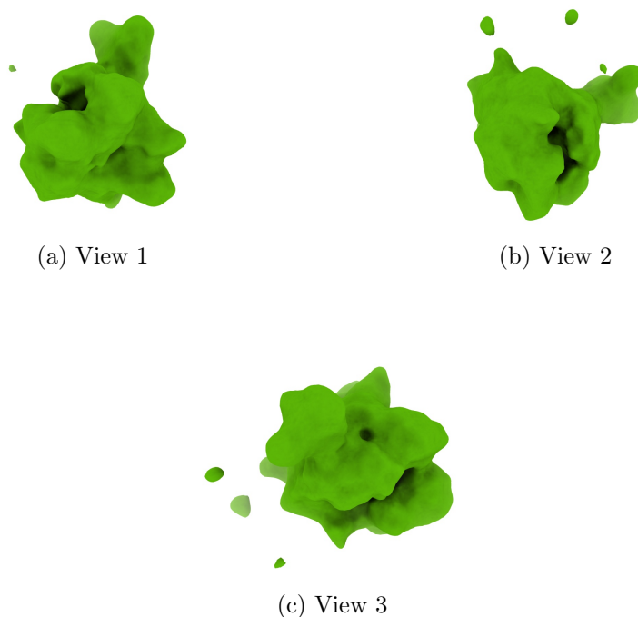
Figure 4: Isosurface at threshold=0.002400. Views generated by ChimeraX at a the following X, Y, Z angles: View 1 (0, -90, -90), View 2 (-90, 0, -90), View 3 (0, 0, 0).
