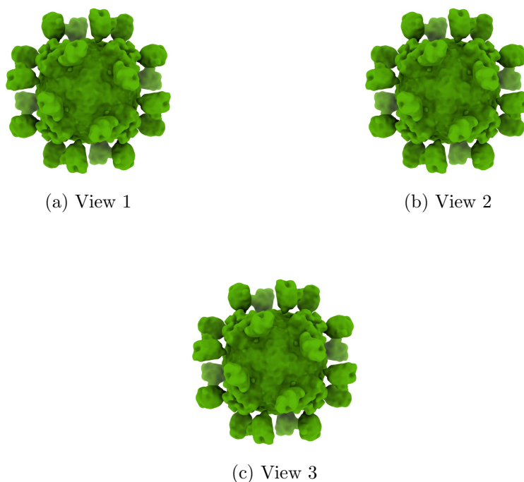
Figure 4: Isosurface at threshold=0.001720. Views generated by ChimeraX at a the following X, Y, Z angles: View 1 (0, -90, -90), View 2 (-90, 0, -90), View 3 (0, 0, 0).
