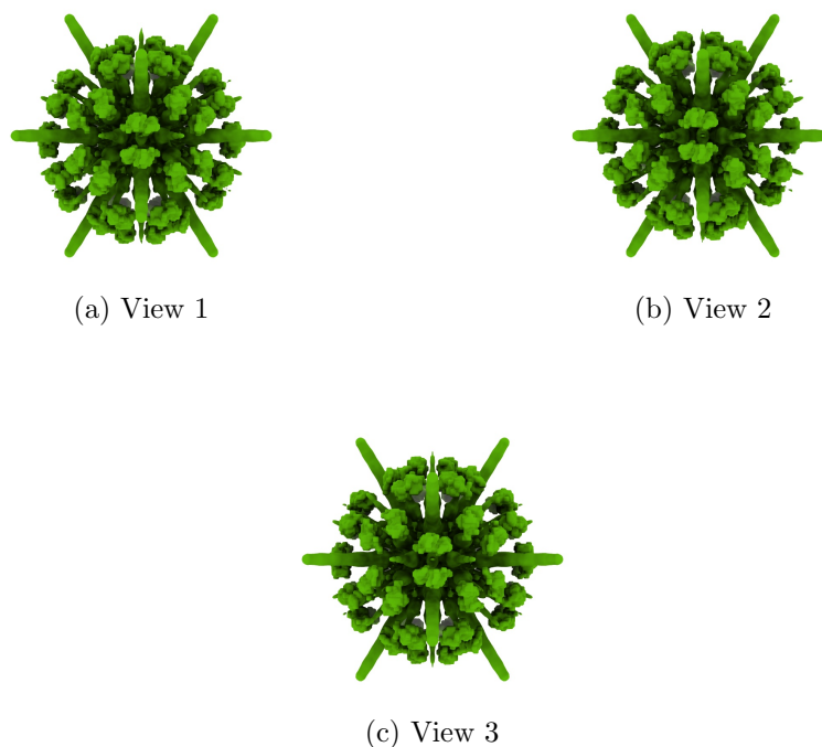
Figure 4: Isosurface at threshold=0.000001. Views generated by ChimeraX at a the following X, Y, Z angles: View 1 (0, -90, -90), View 2 (-90, 0, -90), View 3 (0, 0, 0).
