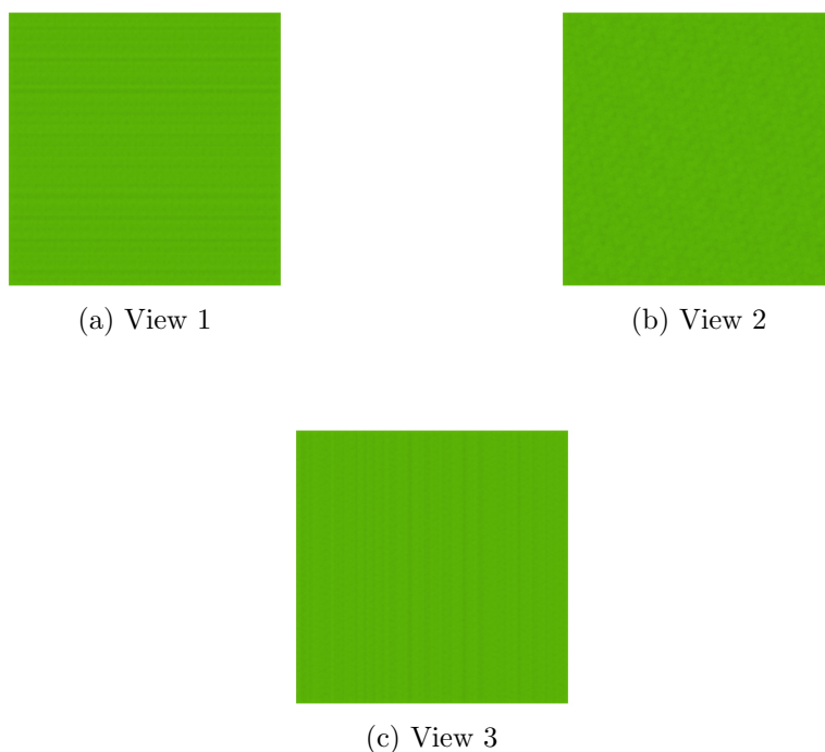
Figure 4: Isosurface at threshold=0.000000. Views generated by ChimeraX at a the following X, Y, Z angles: View 1 (0, -90, -90), View 2 (-90, 0, -90), View 3 (0, 0, 0).
