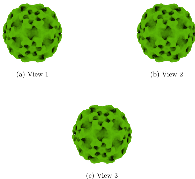
Figure 4: Isosurface at threshold=0.000100. Views generated by ChimeraX at a the following X, Y, Z angles: View 1 (0, -90, -90), View 2 (-90, 0, -90), View 3 (0, 0, 0).
