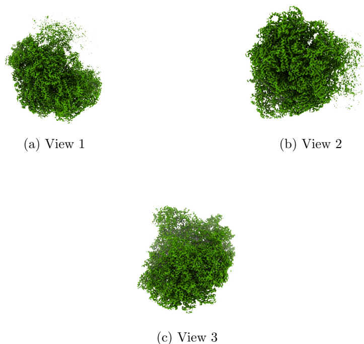
Figure 4: Isosurface at threshold=0.231000. Views generated by ChimeraX at a the following X, Y, Z angles: View 1 (0, -90, -90), View 2 (-90, 0, -90), View 3 (0, 0, 0).
