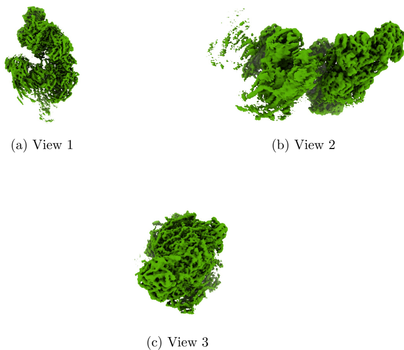
Figure 4: Isosurface at threshold=0.477000. Views generated by ChimeraX at a the following X, Y, Z angles: View 1 (0, -90, -90), View 2 (-90, 0, -90), View 3 (0, 0, 0).
