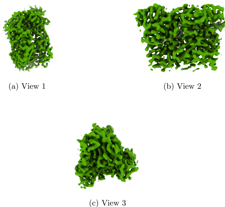
Figure 4: Isosurface at threshold=0.885000. Views generated by ChimeraX at a the following X, Y, Z angles: View 1 (0, -90, -90), View 2 (-90, 0, -90), View 3 (0, 0, 0).
