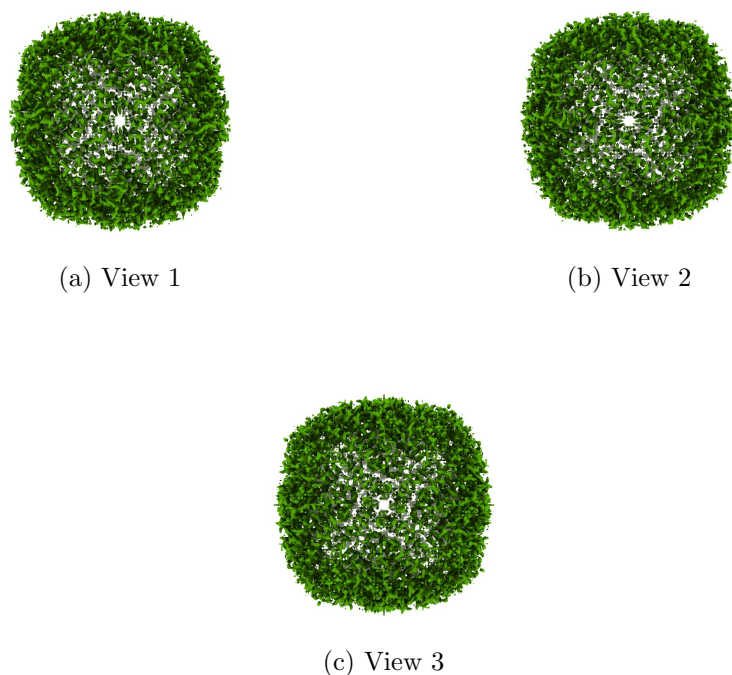
Figure 4: Isosurface at threshold=0.093600. Views generated by ChimeraX at a the following X, Y, Z angles: View 1 (0, -90, -90), View 2 (-90, 0, -90), View 3 (0, 0, 0).
