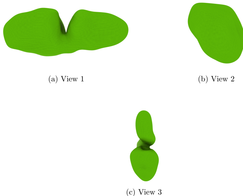
Figure 4: Isosurface at threshold=0.036300. Views generated by ChimeraX at a the following X, Y, Z angles: View 1 (0, -90, -90), View 2 (-90, 0, -90), View 3 (0, 0, 0).
