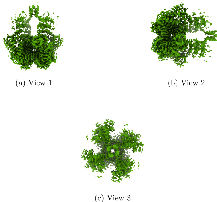
Figure 4: Isosurface at threshold=0.181000. Views generated by ChimeraX at a the following X, Y, Z angles: View 1 (0, -90, -90), View 2 (-90, 0, -90), View 3 (0, 0, 0).
