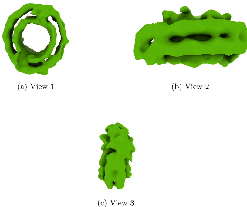
Figure 4: Isosurface at threshold=0.055000. Views generated by ChimeraX at a the following X, Y, Z angles: View 1 (0, -90, -90), View 2 (-90, 0, -90), View 3 (0, 0, 0).
