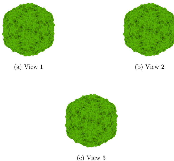
Figure 4: Isosurface at threshold=3289.000000. Views generated by ChimeraX at the following X, Y, Z angles: View 1 (0, -90, -90), View 2 (-90, 0, -90), View 3 (0, 0, 0).
