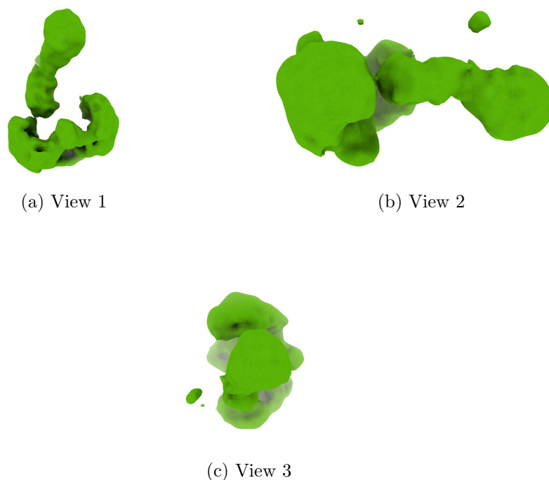
Figure 4: Isosurface at threshold=0.075800. Views generated by ChimeraX at a the following X, Y, Z angles: View 1 (0, -90, -90), View 2 (-90, 0, -90), View 3 (0, 0, 0).
