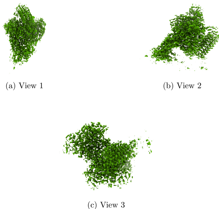
Figure 4: Isosurface at threshold=0.509000. Views generated by ChimeraX at a the following X, Y, Z angles: View 1 (0, -90, -90), View 2 (-90, 0, -90), View 3 (0, 0, 0).
