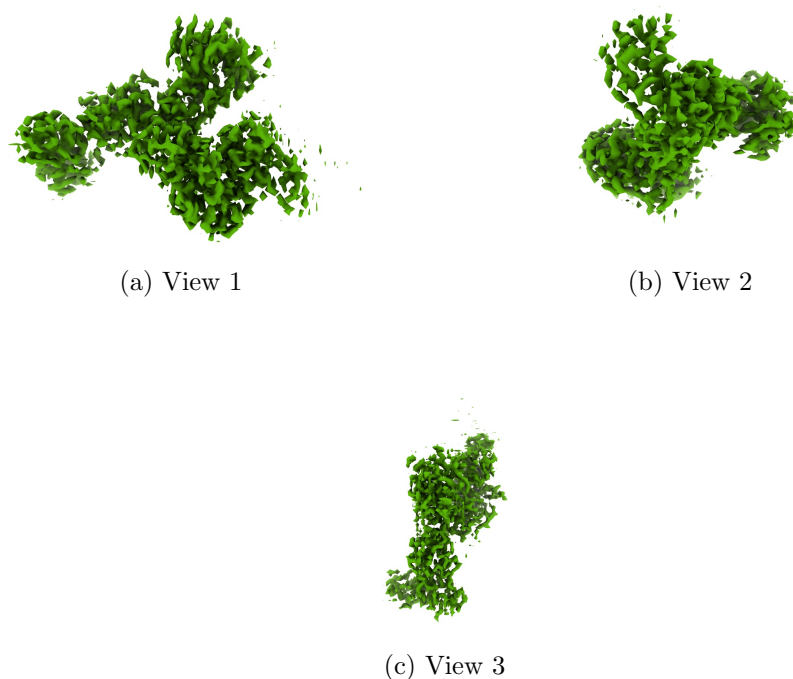
Figure 4: Isosurface at threshold=0.551000. Views generated by ChimeraX at a the following X, Y, Z angles: View 1 (0, -90, -90), View 2 (-90, 0, -90), View 3 (0, 0, 0).
