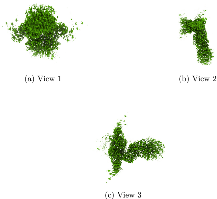
Figure 4: Isosurface at threshold=0.379000. Views generated by ChimeraX at a the following X, Y, Z angles: View 1 (0, -90, -90), View 2 (-90, 0, -90), View 3 (0, 0, 0).
