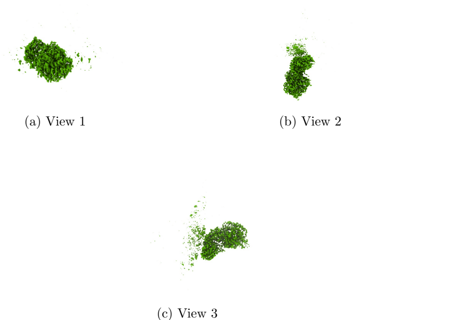
Figure 4: Isosurface at threshold=0.307000. Views generated by ChimeraX at a the following X, Y, Z angles: View 1 (0, -90, -90), View 2 (-90, 0, -90), View 3 (0, 0, 0).
