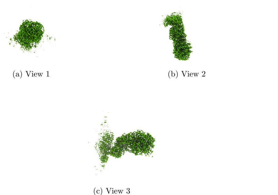
Figure 4: Isosurface at threshold=0.430000. Views generated by ChimeraX at a the following X, Y, Z angles: View 1 (0, -90, -90), View 2 (-90, 0, -90), View 3 (0, 0, 0).
