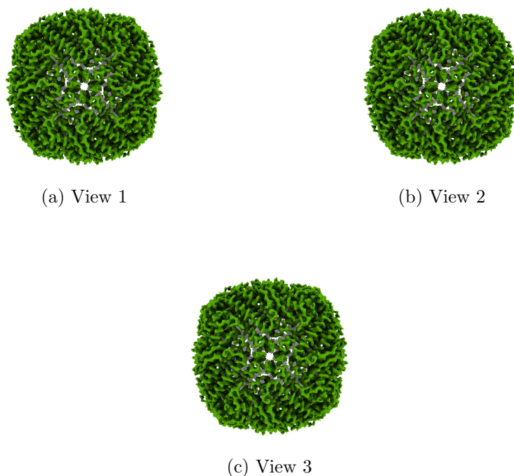
Figure 4: Isosurface at threshold=0.004690. Views generated by ChimeraX at a the following X, Y, Z angles: View 1 (0, -90, -90), View 2 (-90, 0, -90), View 3 (0, 0, 0).
