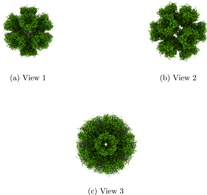
Figure 4: Isosurface at threshold=0.019900. Views generated by ChimeraX at a the following X, Y, Z angles: View 1 (0, -90, -90), View 2 (-90, 0, -90), View 3 (0, 0, 0).
