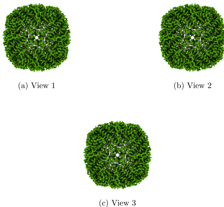
Figure 4: Isosurface at threshold=0.004080. Views generated by ChimeraX at a the following X, Y, Z angles: View 1 (0, -90, -90), View 2 (-90, 0, -90), View 3 (0, 0, 0).
