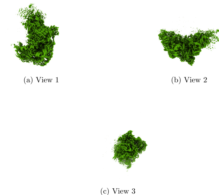
Figure 4: Isosurface at threshold=0.283000. Views generated by ChimeraX at a the following X, Y, Z angles: View 1 (0, -90, -90), View 2 (-90, 0, -90), View 3 (0, 0, 0).
