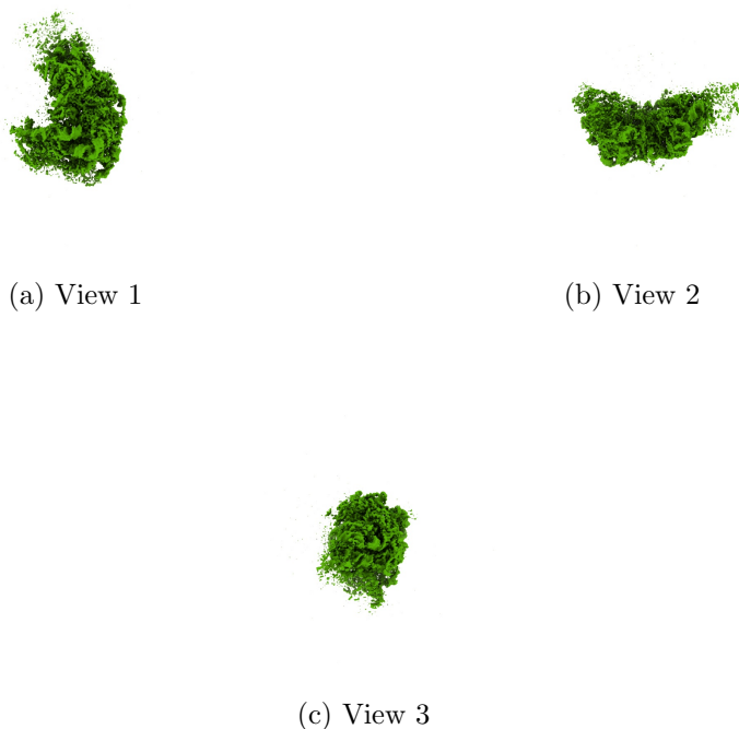
Figure 4: Isosurface at threshold=0.281000. Views generated by ChimeraX at a the following X, Y, Z angles: View 1 (0, -90, -90), View 2 (-90, 0, -90), View 3 (0, 0, 0).
