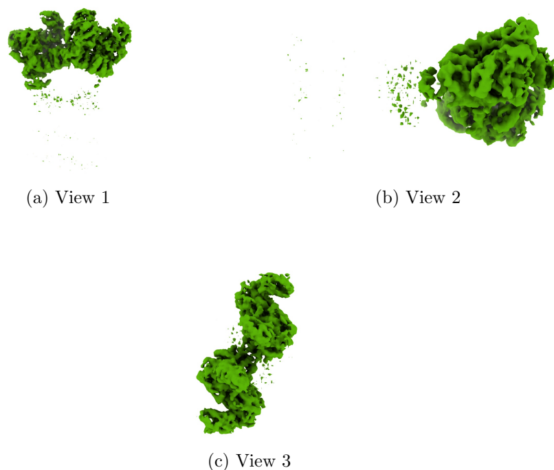
Figure 4: Isosurface at threshold=0.288000. Views generated by ChimeraX at a the following X, Y, Z angles: View 1 (0, -90, -90), View 2 (-90, 0, -90), View 3 (0, 0, 0).
