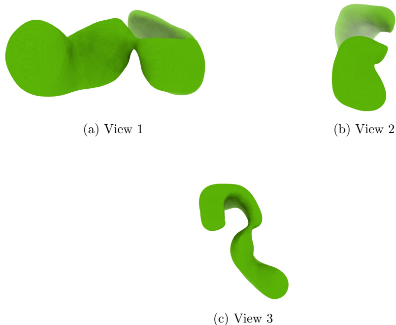
Figure 4: Isosurface at threshold=0.072100. Views generated by ChimeraX at a the following X, Y, Z angles: View 1 (0, -90, -90), View 2 (-90, 0, -90), View 3 (0, 0, 0).
