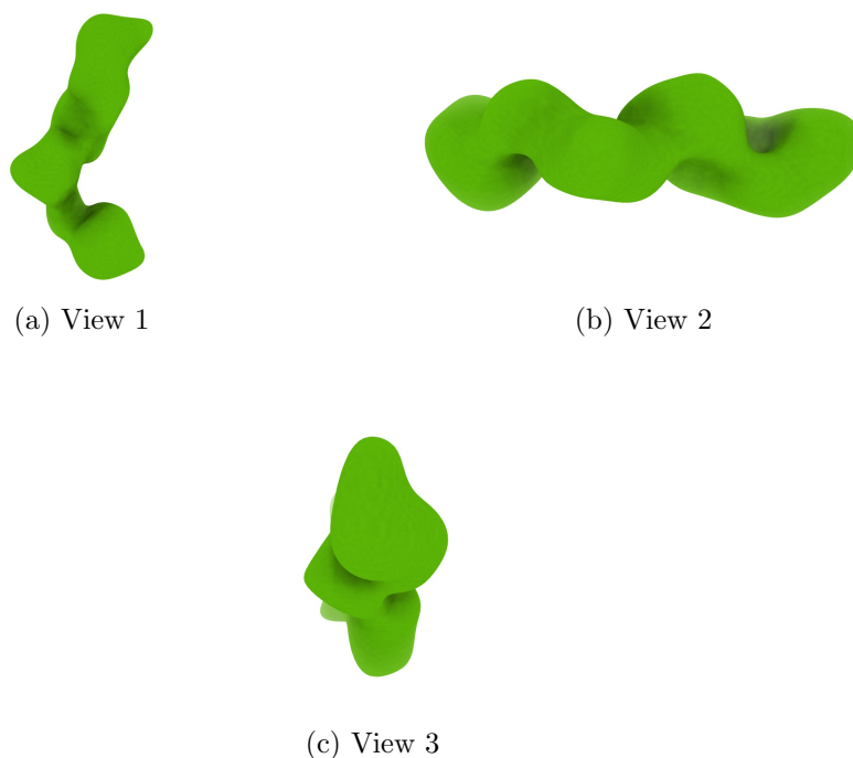
Figure 4: Isosurface at threshold=0.075500. Views generated by ChimeraX at a the following X, Y, Z angles: View 1 (0, -90, -90), View 2 (-90, 0, -90), View 3 (0, 0, 0).
