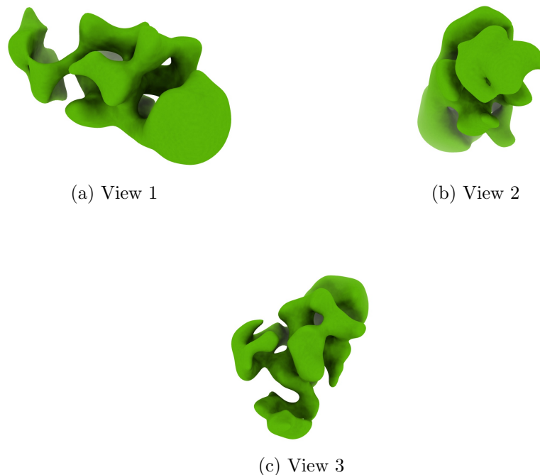
Figure 4: Isosurface at threshold=5.820000. Views generated by ChimeraX at a the following X, Y, Z angles: View 1 (0, -90, -90), View 2 (-90, 0, -90), View 3 (0, 0, 0).
