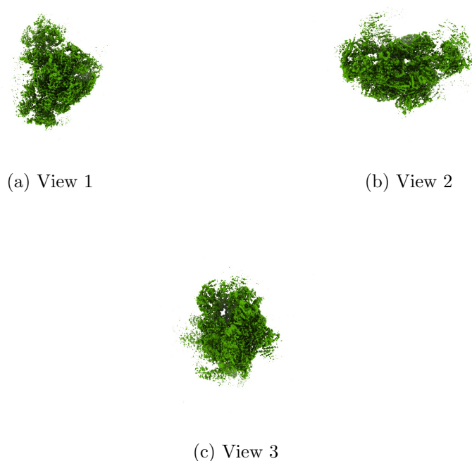
Figure 4: Isosurface at threshold=0.362000. Views generated by ChimeraX at a the following X, Y, Z angles: View 1 (0, -90, -90), View 2 (-90, 0, -90), View 3 (0, 0, 0).
