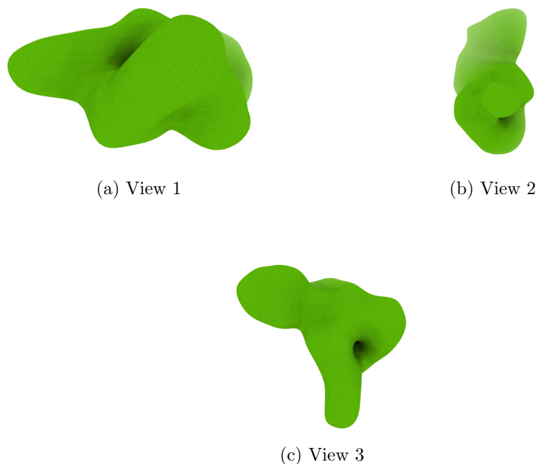
Figure 4: Isosurface at threshold=2.950000. Views generated by ChimeraX at a the following X, Y, Z angles: View 1 (0, -90, -90), View 2 (-90, 0, -90), View 3 (0, 0, 0).
