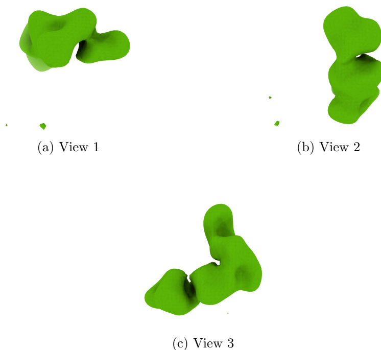
Figure 4: Isosurface at threshold=5.130000. Views generated by ChimeraX at a the following X, Y, Z angles: View 1 (0, -90, -90), View 2 (-90, 0, -90), View 3 (0, 0, 0).
