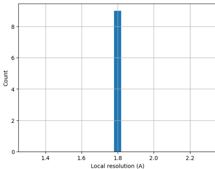
Figure 24: Histogram of the local resolution according to Resmap.
