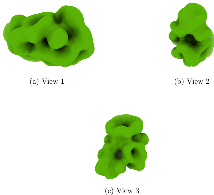
Figure 4: Isosurface at threshold=0.012600. Views generated by ChimeraX at a the following X, Y, Z angles: View 1 (0, -90, -90), View 2 (-90, 0, -90), View 3 (0, 0, 0).
