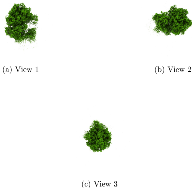
Figure 4: Isosurface at threshold=0.139000. Views generated by ChimeraX at a the following X, Y, Z angles: View 1 (0, -90, -90), View 2 (-90, 0, -90), View 3 (0, 0, 0).
