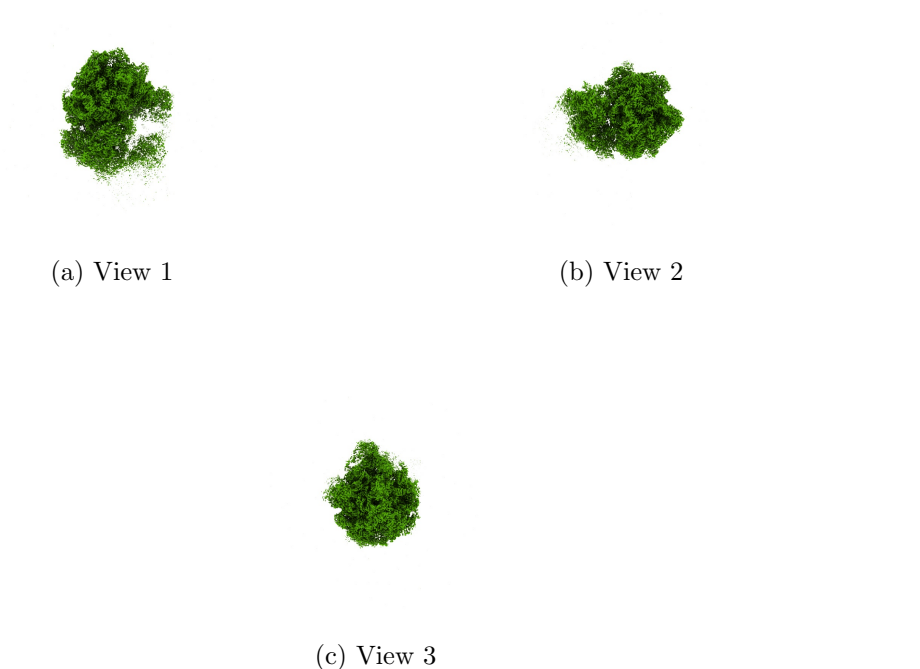
Figure 4: Isosurface at threshold=0.136000. Views generated by ChimeraX at a the following X, Y, Z angles: View 1 (0, -90, -90), View 2 (-90, 0, -90), View 3 (0, 0, 0).
