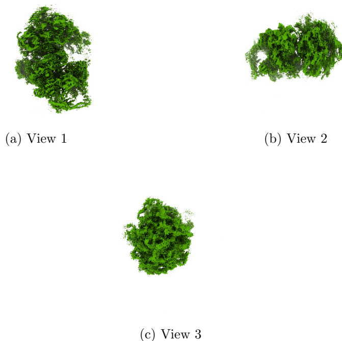
Figure 4: Isosurface at threshold=0.066200. Views generated by ChimeraX at a the following X, Y, Z angles: View 1 (0, -90, -90), View 2 (-90, 0, -90), View 3 (0, 0, 0).
