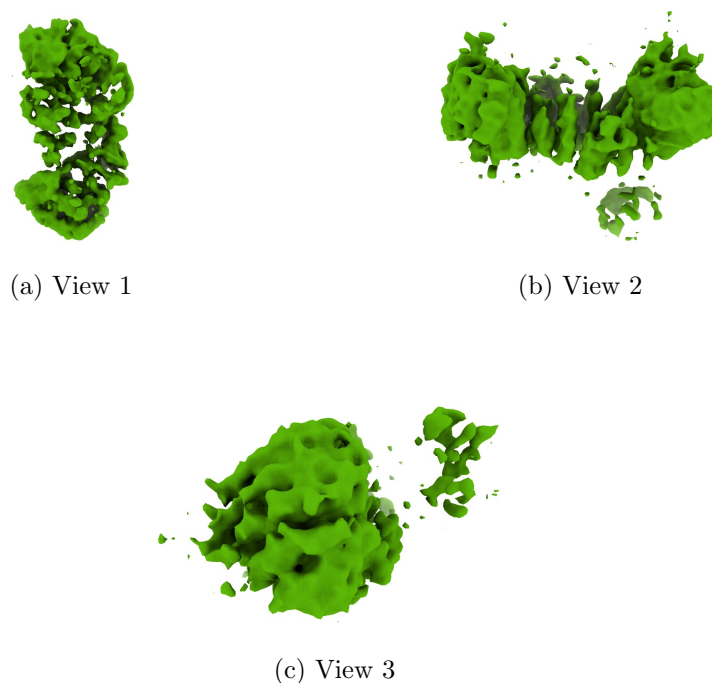
Figure 4: Isosurface at threshold=0.073400. Views generated by ChimeraX at a the following X, Y, Z angles: View 1 (0, -90, -90), View 2 (-90, 0, -90), View 3 (0, 0, 0).
