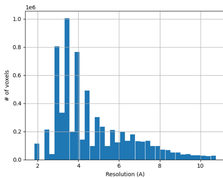
Figure 25: Histogram of the local resolution according to MonoRes.
