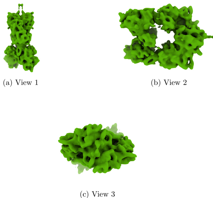
Figure 4: Isosurface at threshold=13.800000. Views generated by ChimeraX at a the following X, Y, Z angles: View 1 (0, -90, -90), View 2 (-90, 0, -90), View 3 (0, 0, 0).
