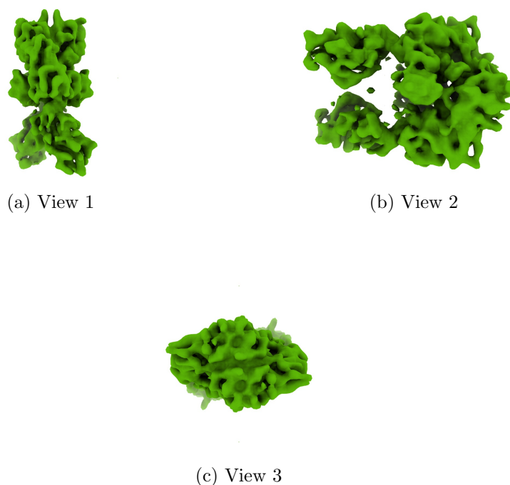
Figure 4: Isosurface at threshold=7.300000. Views generated by ChimeraX at a the following X, Y, Z angles: View 1 (0, -90, -90), View 2 (-90, 0, -90), View 3 (0, 0, 0).
