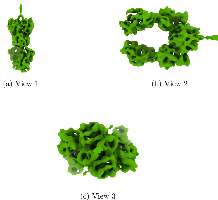
Figure 4: Isosurface at threshold=8.700000. Views generated by ChimeraX at a the following X, Y, Z angles: View 1 (0, -90, -90), View 2 (-90, 0, -90), View 3 (0, 0, 0).
