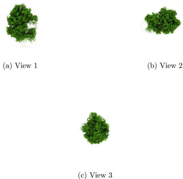
Figure 4: Isosurface at threshold=0.131000. Views generated by ChimeraX at a the following X, Y, Z angles: View 1 (0, -90, -90), View 2 (-90, 0, -90), View 3 (0, 0, 0).
