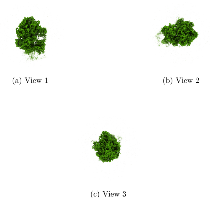
Figure 4: Isosurface at threshold=0.090900. Views generated by ChimeraX at a the following X, Y, Z angles: View 1 (0, -90, -90), View 2 (-90, 0, -90), View 3 (0, 0, 0).
