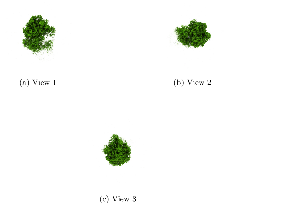
Figure 4: Isosurface at threshold=0.139000. Views generated by ChimeraX at a the following X, Y, Z angles: View 1 (0, -90, -90), View 2 (-90, 0, -90), View 3 (0, 0, 0).
