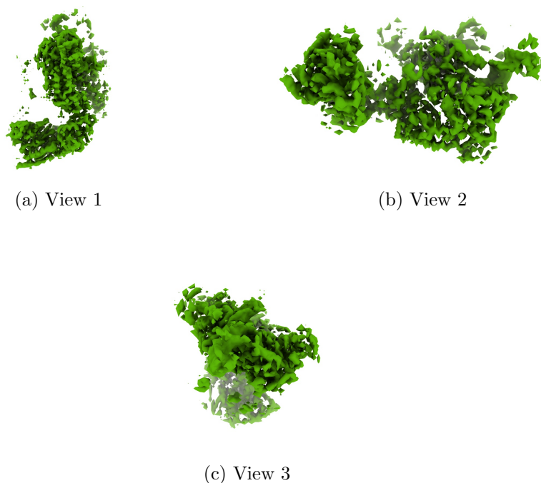
Figure 4: Isosurface at threshold=0.012700. Views generated by ChimeraX at a the following X, Y, Z angles: View 1 (0, -90, -90), View 2 (-90, 0, -90), View 3 (0, 0, 0).
