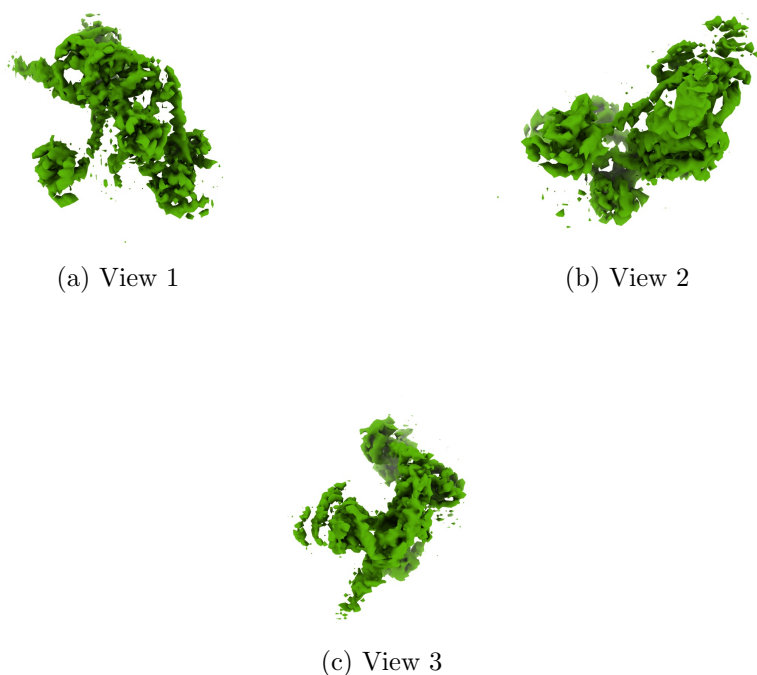
Figure 4: Isosurface at threshold=0.010200. Views generated by ChimeraX at a the following X, Y, Z angles: View 1 (0, -90, -90), View 2 (-90, 0, -90), View 3 (0, 0, 0).
