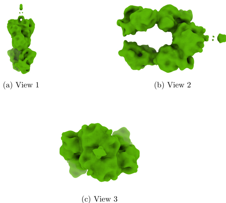
Figure 4: Isosurface at threshold=6.200000. Views generated by ChimeraX at a the following X, Y, Z angles: View 1 (0, -90, -90), View 2 (-90, 0, -90), View 3 (0, 0, 0).
