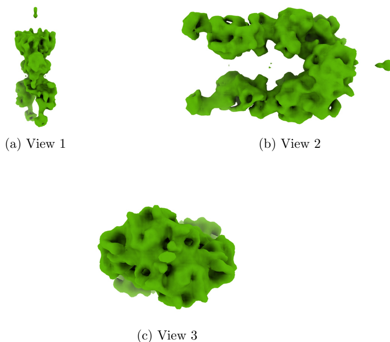
Figure 4: Isosurface at threshold=7.200000. Views generated by ChimeraX at a the following X, Y, Z angles: View 1 (0, -90, -90), View 2 (-90, 0, -90), View 3 (0, 0, 0).
